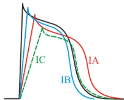
Ventricular Action Potential
