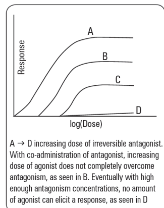
Figure 7. The log(dose)-response curve for irreversible antagonism
