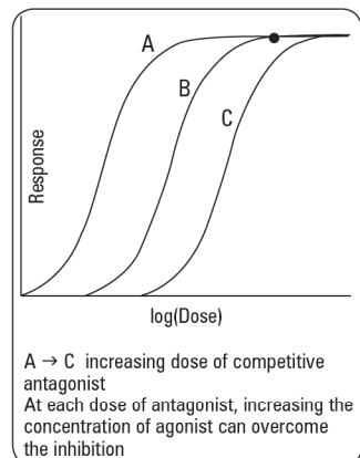
Figure 6. The log(dose)-response curve for competitive reversible antagonism
